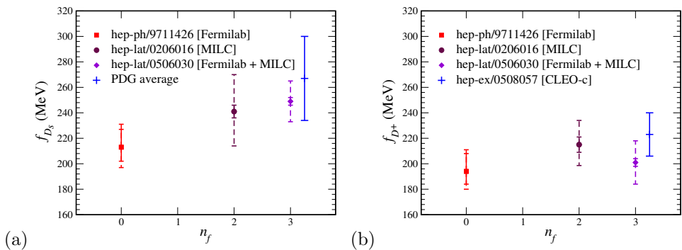
Fig. 2. Dependence of (a) f_{D_s} and (b) f_{D^+} on the number n_f of sea flavors. Quenched ( n_f = 0 ) 18 ; n_f = 2 19 ; n_f = 3 15 . Solid (dashed) error bars are statistical (statistical+systematic).
