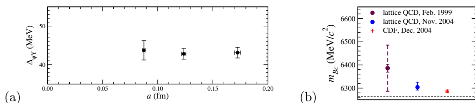
Fig. 3. (a) Dependence of the splitting \Delta_{\psi\Upsilon} on the lattice spacing a . (b) Comparison of the quenched 26 , n_f = 2 + 1 24 , and experimental 25 values of m_{B_c} ; the dashed line denotes the baseline (\bar{m}_\psi + m_\Upsilon)/2 .
