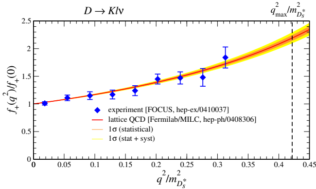
Fig. 1. Shape of form factor f_+(q^2)/f_+(0) vs. q^2/m_{D_s^*}^2 , compared with experiment 10 .
