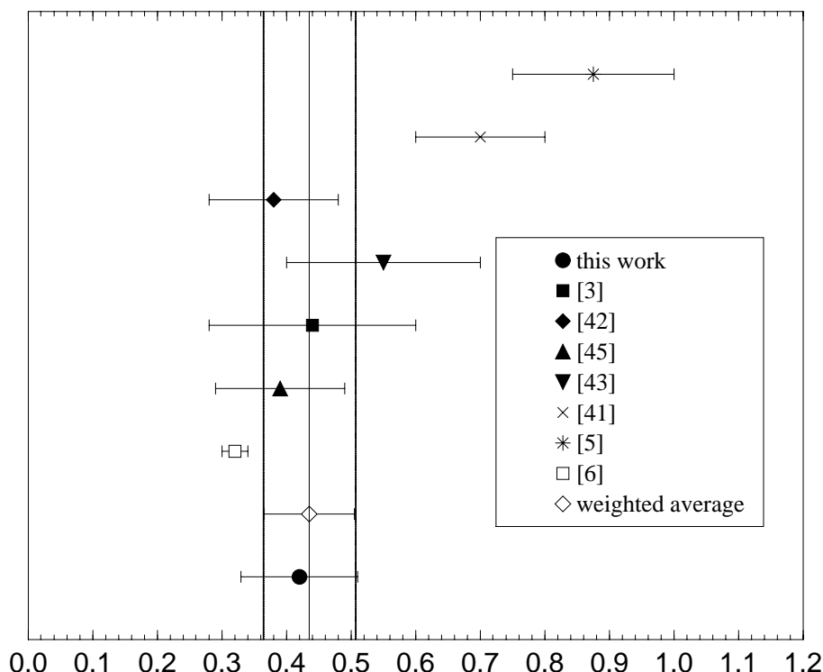
Figure 7: Comparison of various estimates of the coupling g .
