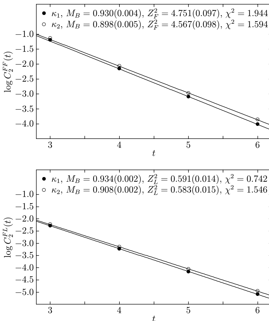
Figure 2: Logarithmic plots of C_2^{FF}(t) and C_2^{FL}(t) for both values of \kappa . The quoted values refer to the reduced \chi^2 .
