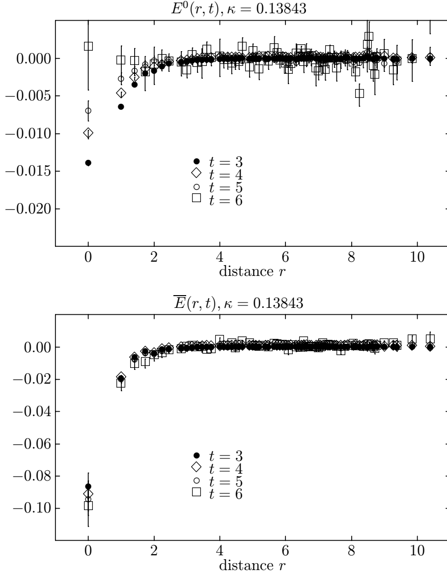
Figure 3: Plots of E^0(r, t) and \overline{E}(r, t) as functions of r for different values of t ( = 3, 4, 5, 6 ) for \kappa = 0.13843 .
