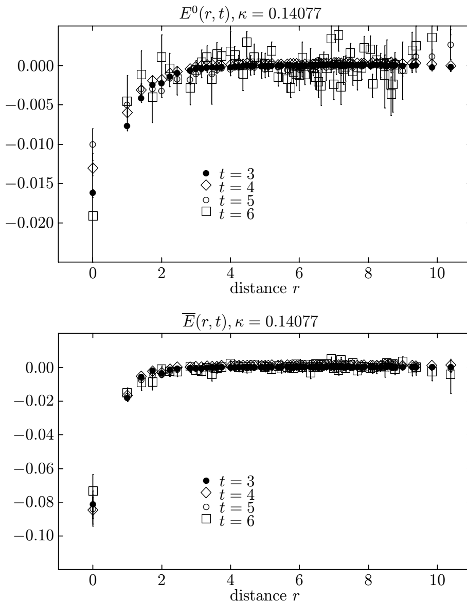
Figure 4: Plots of E^0(r, t) and \overline{E}(r, t) as functions of r for different values of t ( = 3, 4, 5, 6 ) for \kappa = 0.14077 .
